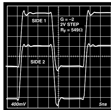
TPC 35. 2 V Step Response, G = -2
